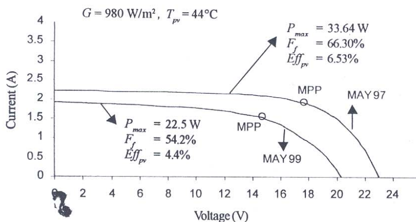
Fig. 6. I - V curves of the amorphous PV-module type 2 measured during the first three years of operation.
