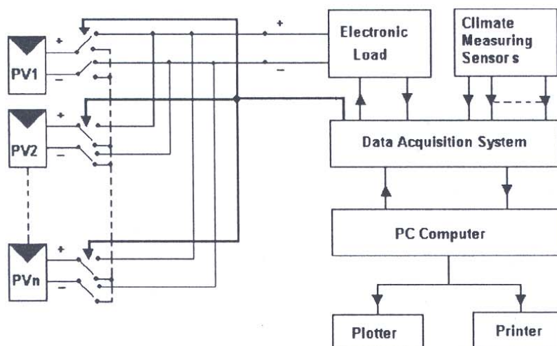
Fig. 3. Automatic system for measuring the I-V characteristic of PV-modules.
