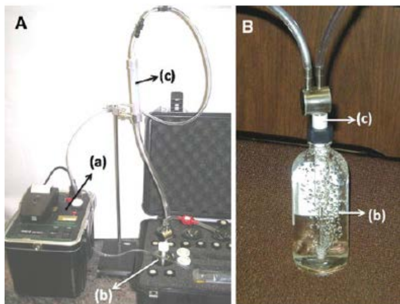
Figure 1 Schematic presentations of radon-in-air monitor RAD-7. Adapted from reference [18] with permission.
